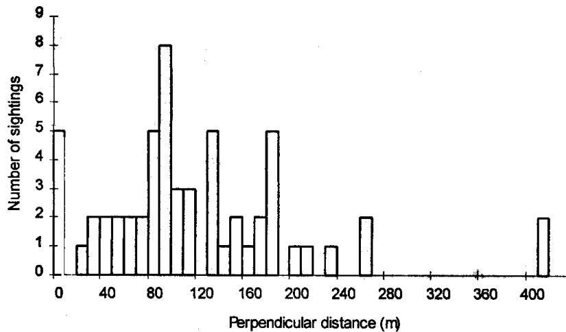
Figure 2. Frequency distribution of perpendicular distance raw data to sightings for dusky dolphin surveys. Cut-points every 10 m.
