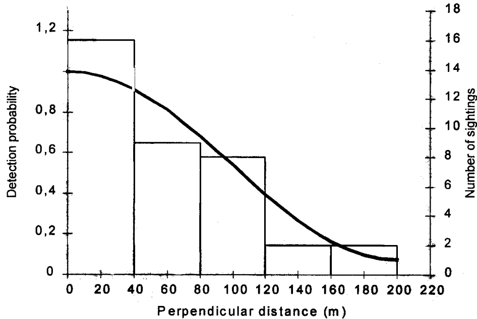
Figure 3. Frequency distribution of perpendicular distances to sightings for dusky dolphin surveys. Data rescaled to left-truncation point of 80 m. Continuous curve represents probability detection function based on fit of Fourier Series to perpendicular-distance data.
